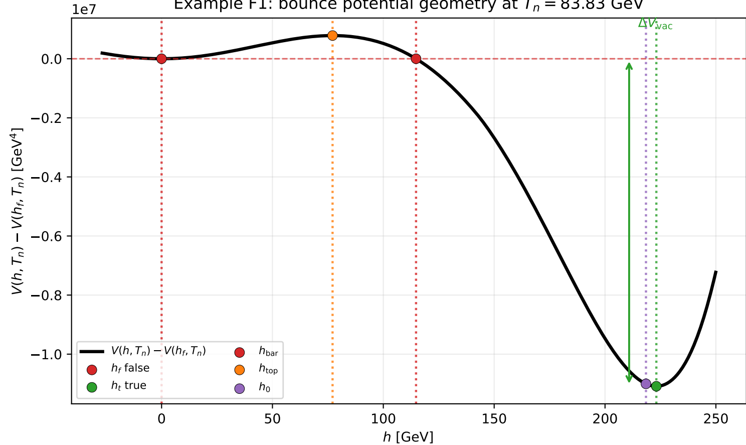
Example F1: bounce potential geometry at T_n = 83.83 GeV
