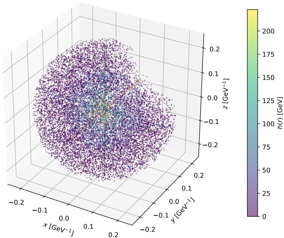
Example F5: 3D bubble profile at T_n = 83.83 GeV
