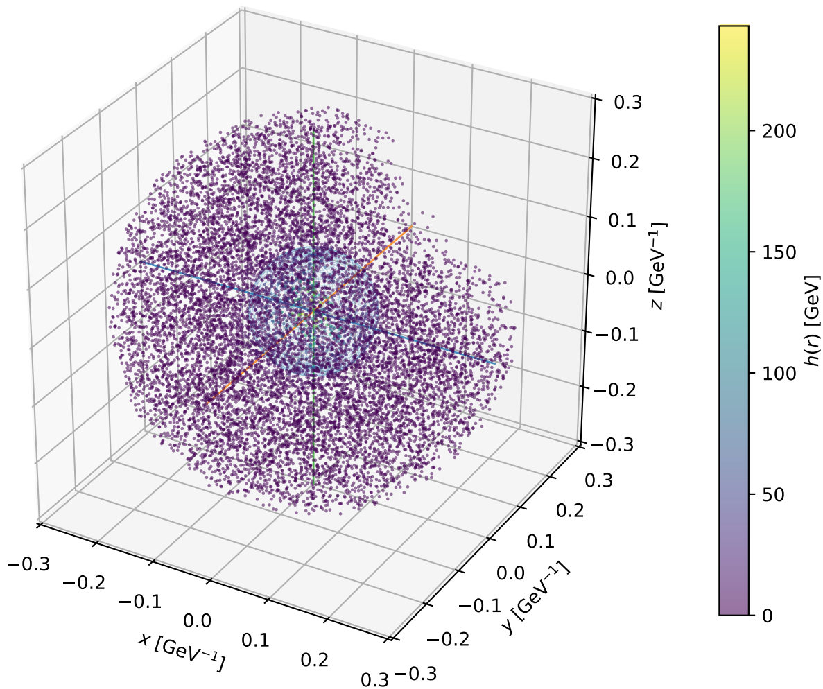
Example F5: 3D bubble profile at T_n = 48.69 GeV
