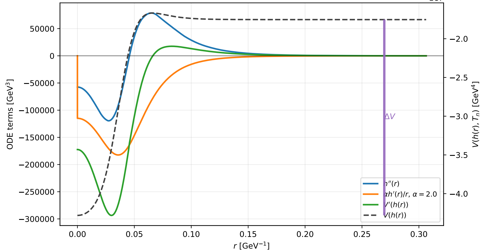
Example F7: bounce equation terms at T_n = 48.69 GeV
