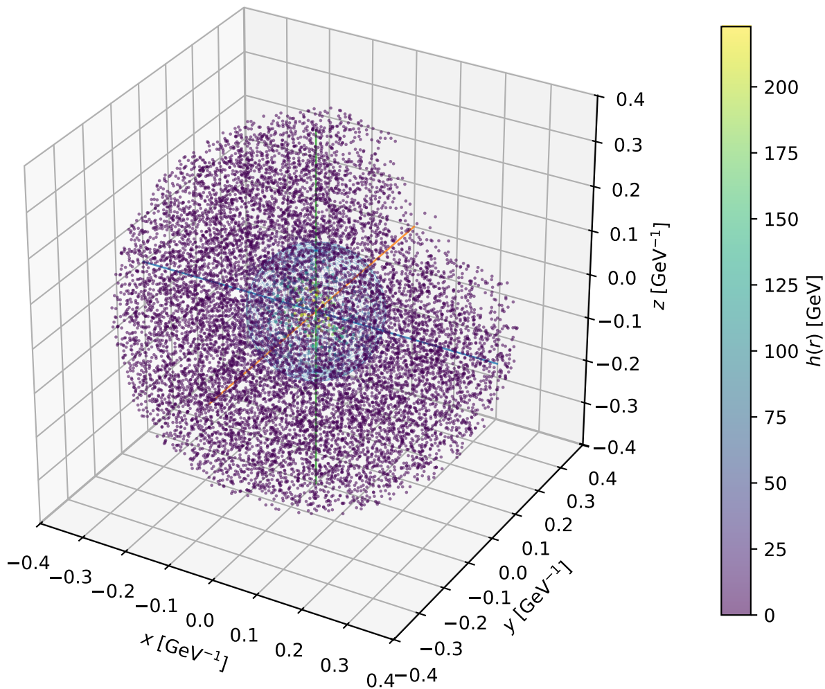
Example F5: 3D bubble profile at T_n = 85.16 GeV
