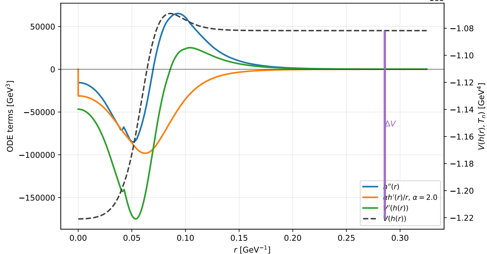
Example F7: bounce equation terms at T_n = 80.64 GeV
