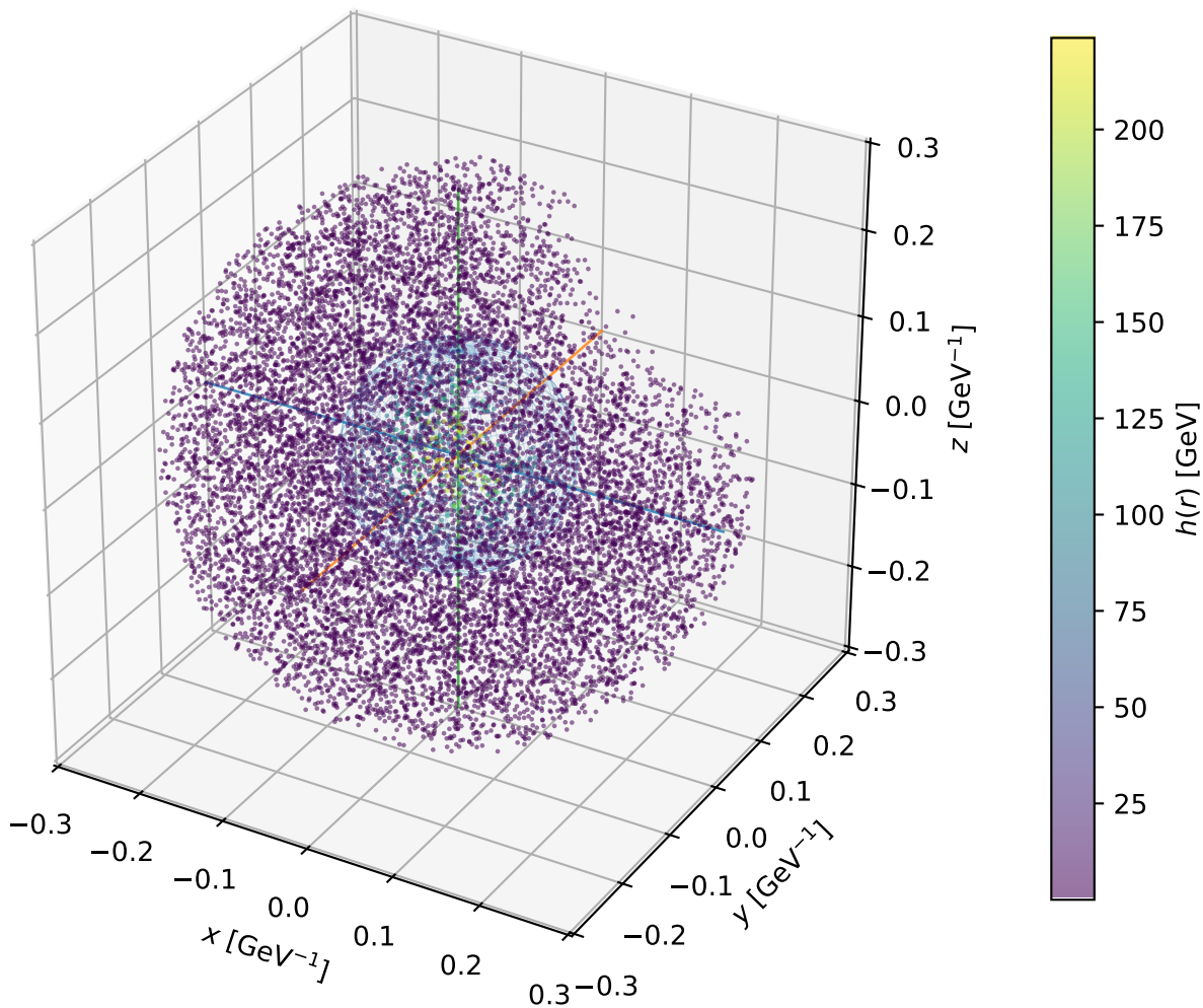
Example F5: 3D bubble profile at T_n = 82.36 GeV
