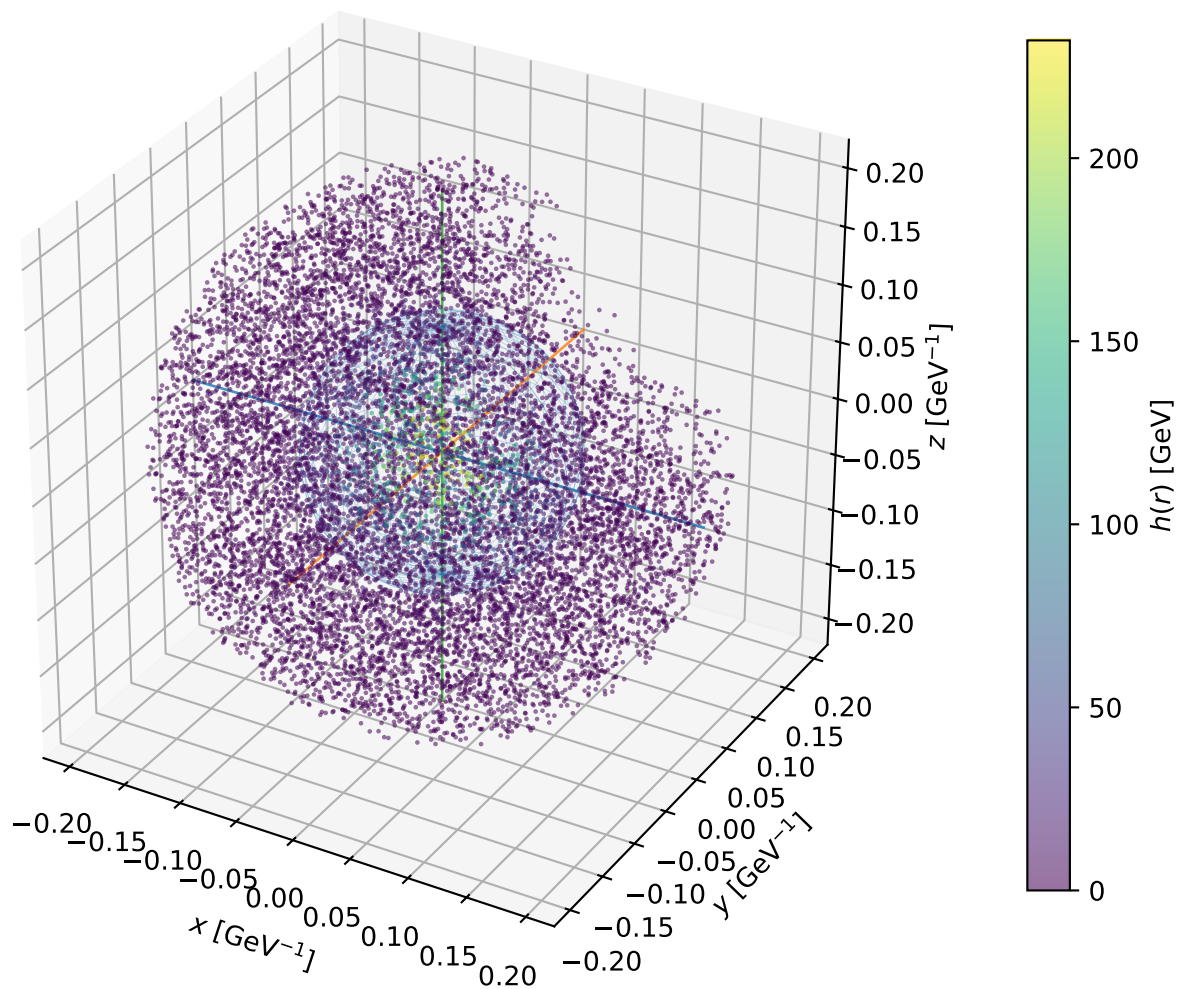
Example F5: 3D bubble profile at T_n = 72.89 GeV
