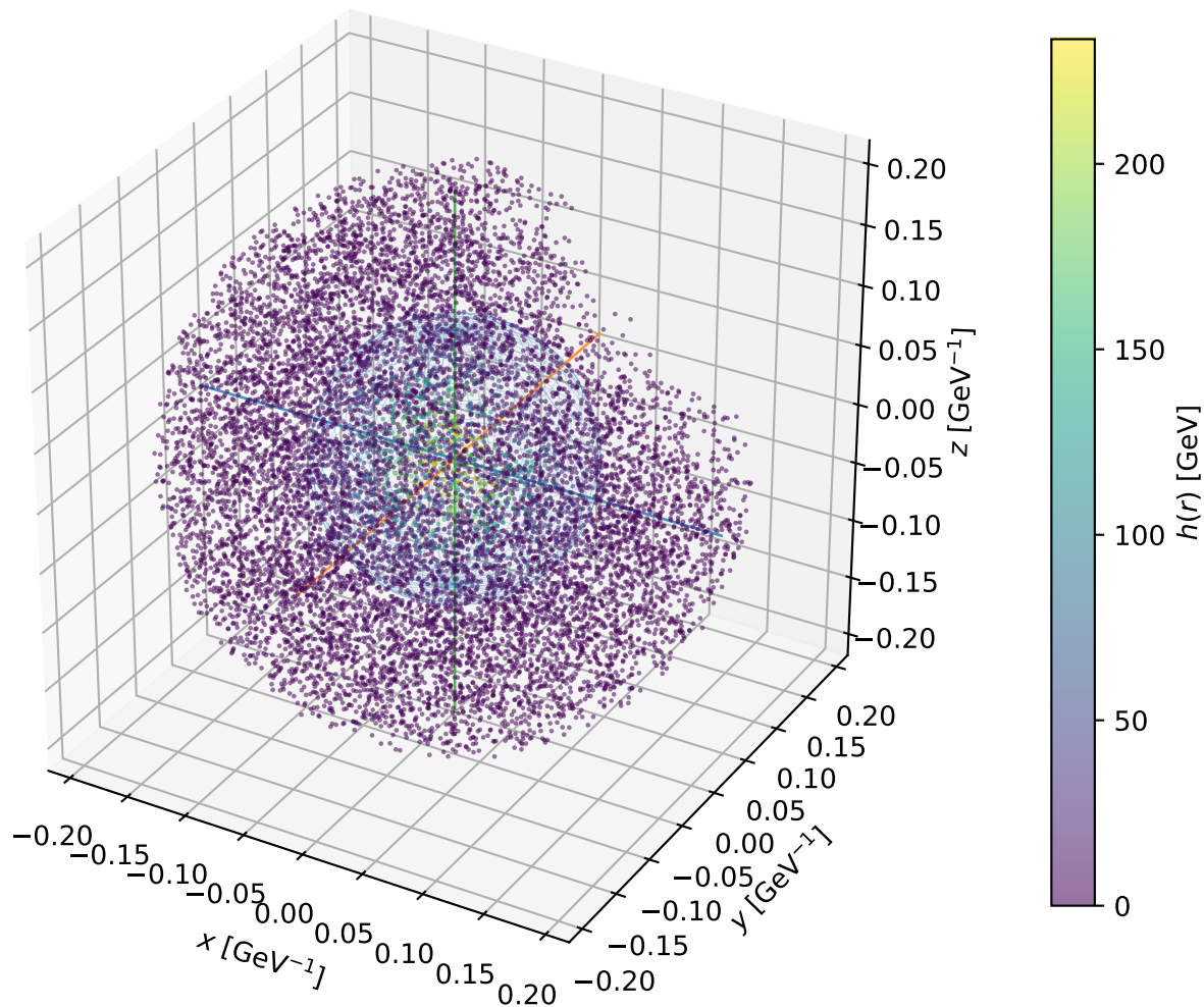
Example F5: 3D bubble profile at T_n = 70.68 GeV
