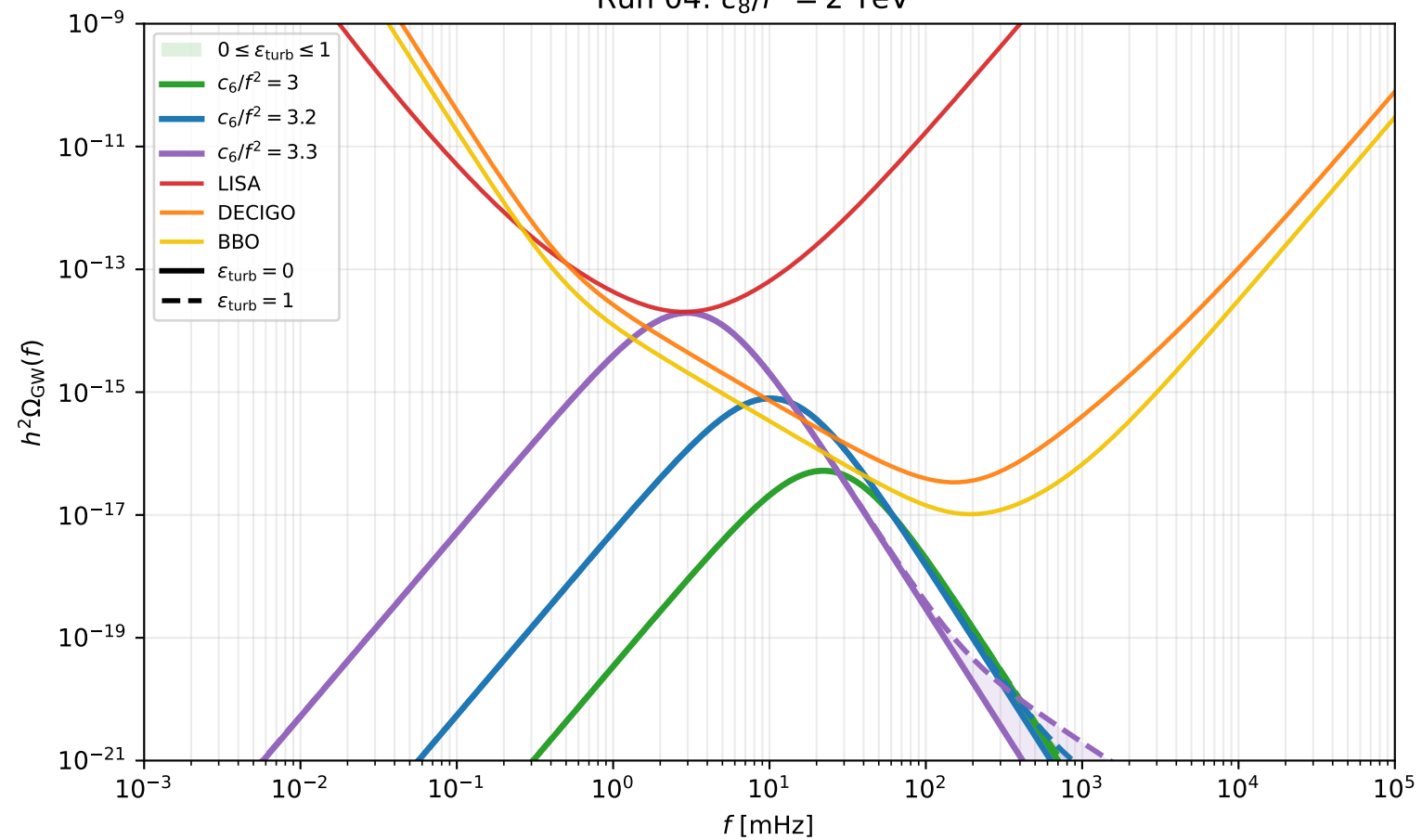
Run 04: c_8/f^4 = 2 \text{ TeV}^{-4}
