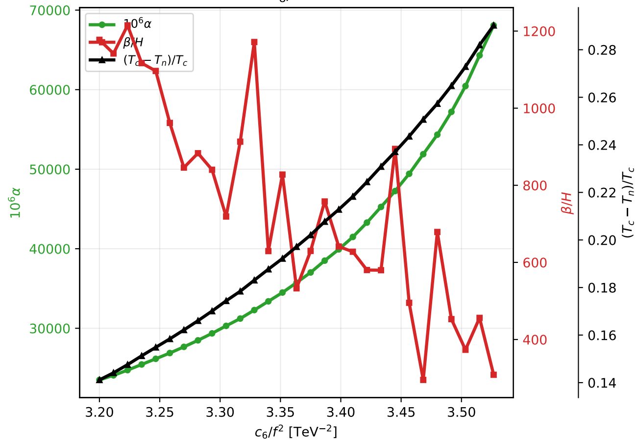
Run 05: c_8/f^4 = 0 \text{ TeV}^{-4}
