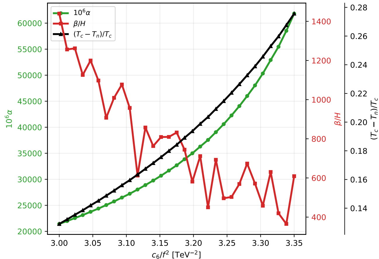
Run 05: c_8/f^4 = 2 \text{ TeV}^{-4}
