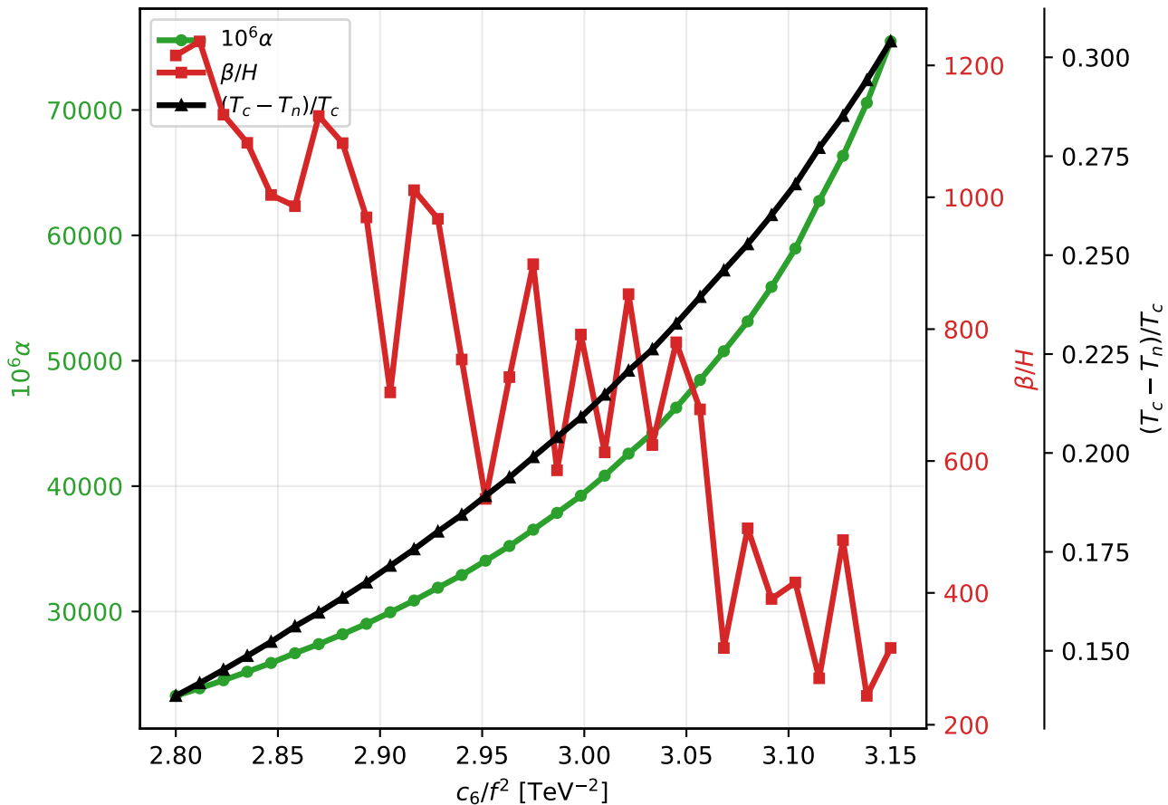
Run 05: c_8/f^4 = 5 \text{ TeV}^{-4}
