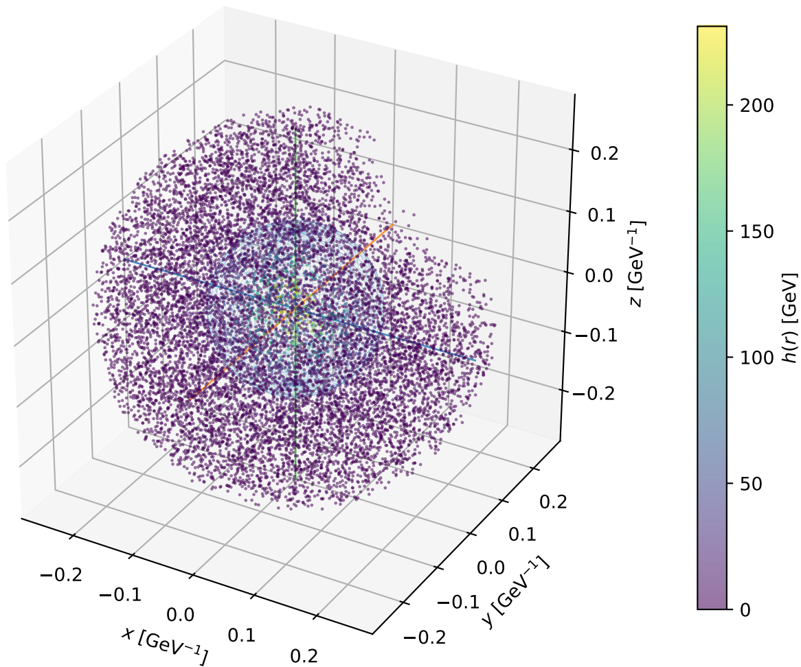
Example F5: 3D bubble profile at T_n = 74.86 GeV
