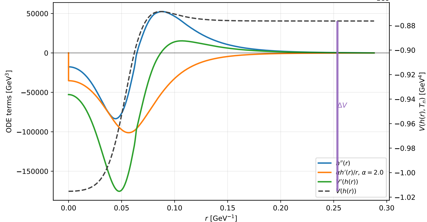
Example F7: bounce equation terms at T_n = 74.86 GeV
