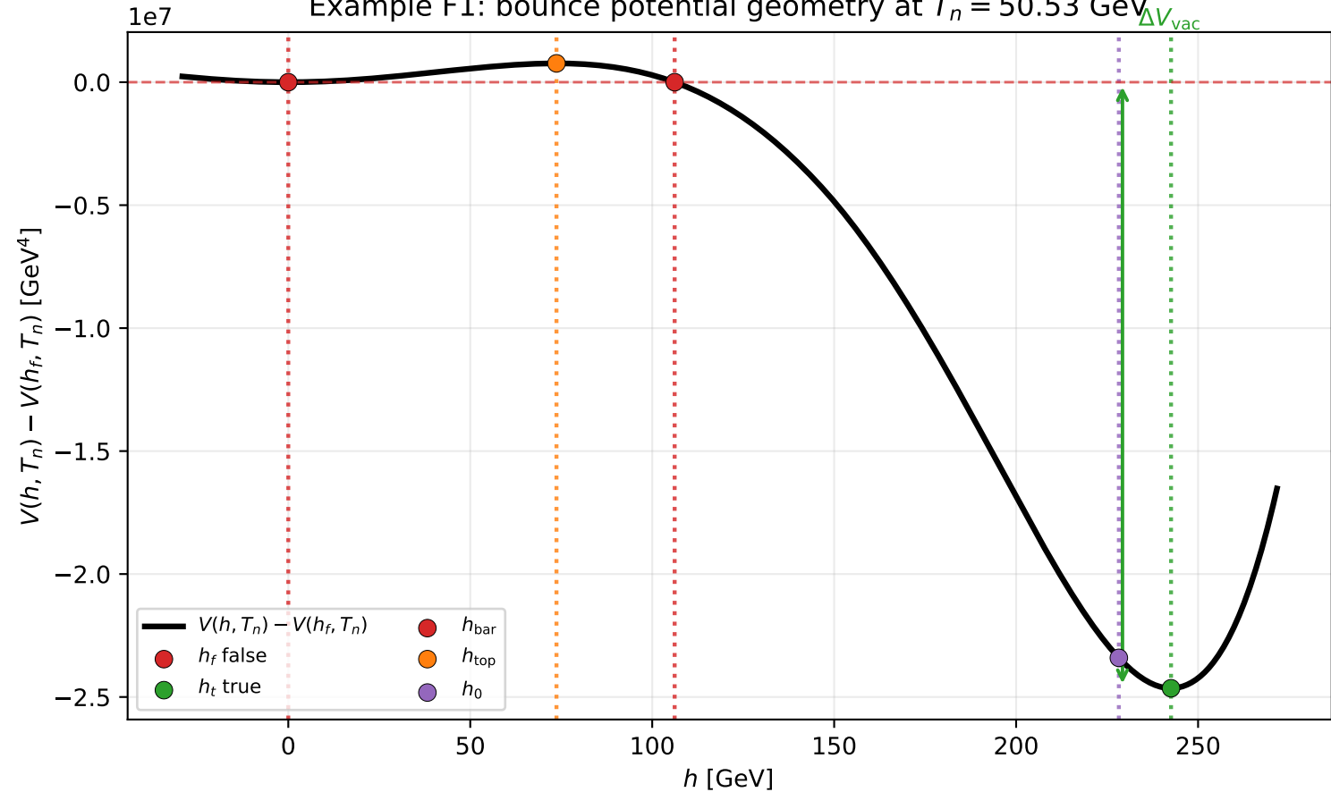
Example F1: bounce potential geometry at T_n = 50.53 GeV
