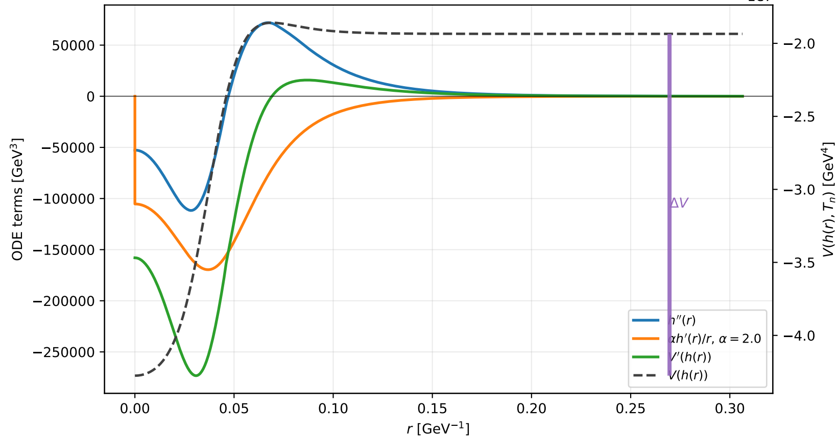
Example F7: bounce equation terms at T_n = 50.53 GeV
