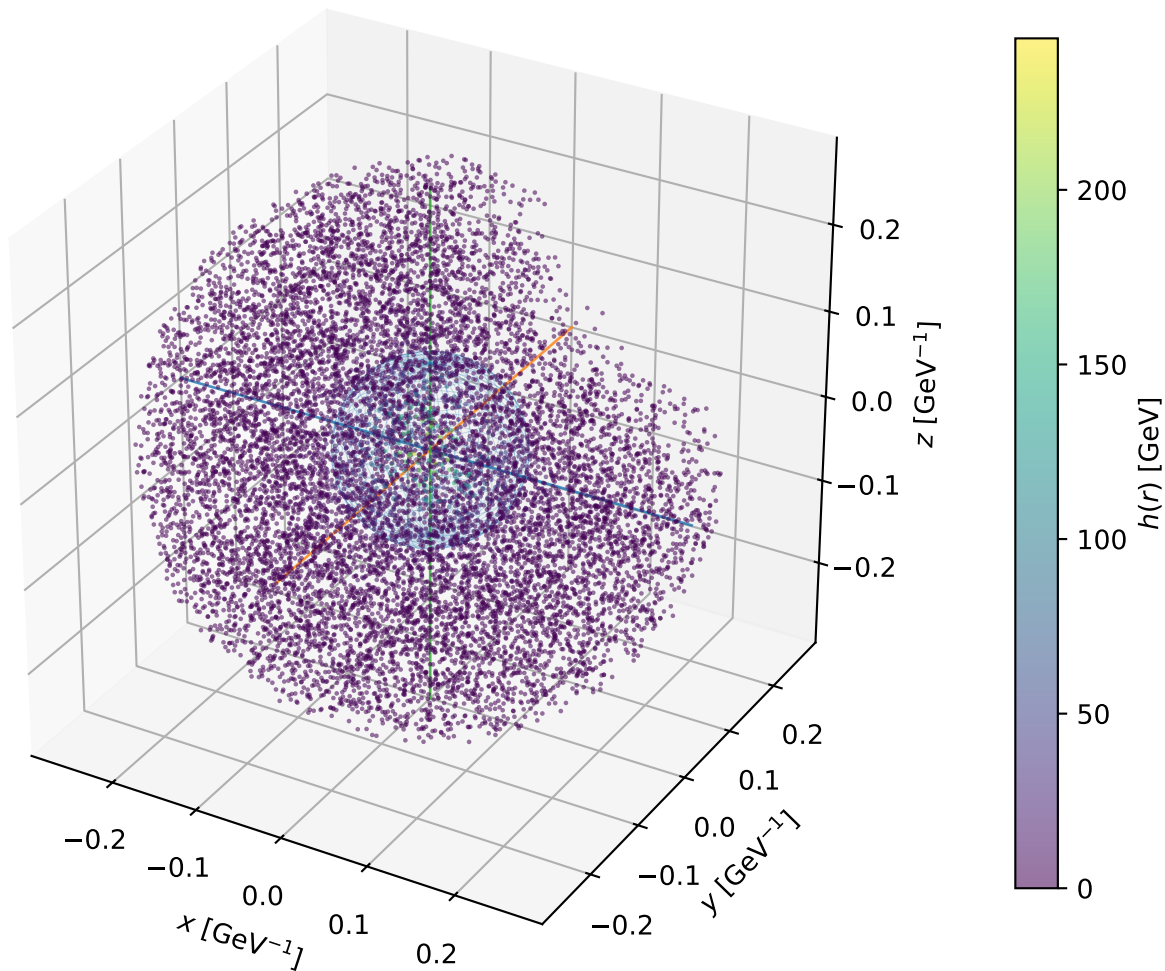
Example F5: 3D bubble profile at T_n = 46.8 GeV
