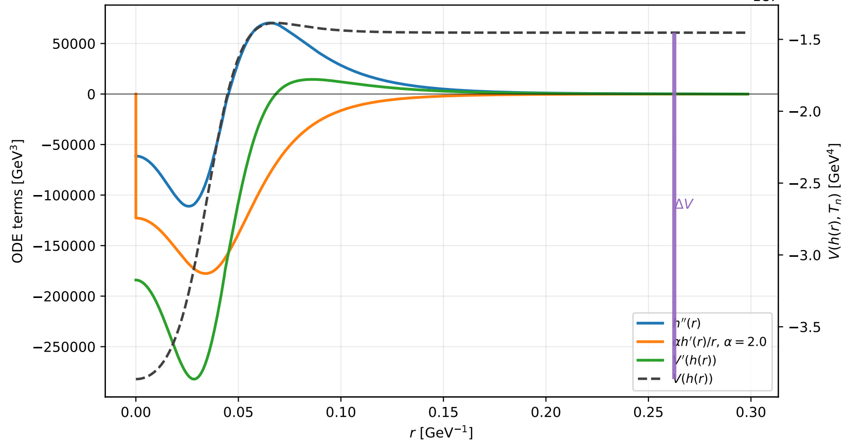
Example F7: bounce equation terms at T_n = 46.8 GeV
