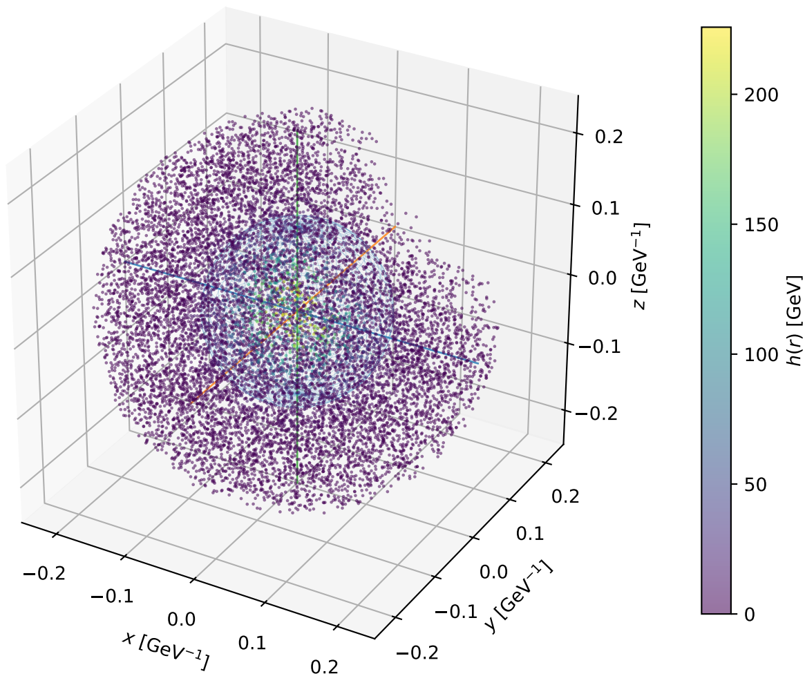
Example F5: 3D bubble profile at T_n = 80.39 GeV
