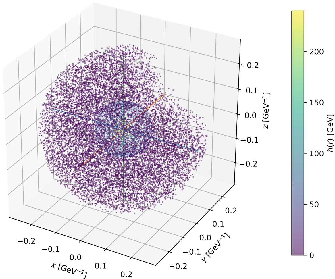
Example F5: 3D bubble profile at T_n = 59.26 GeV
