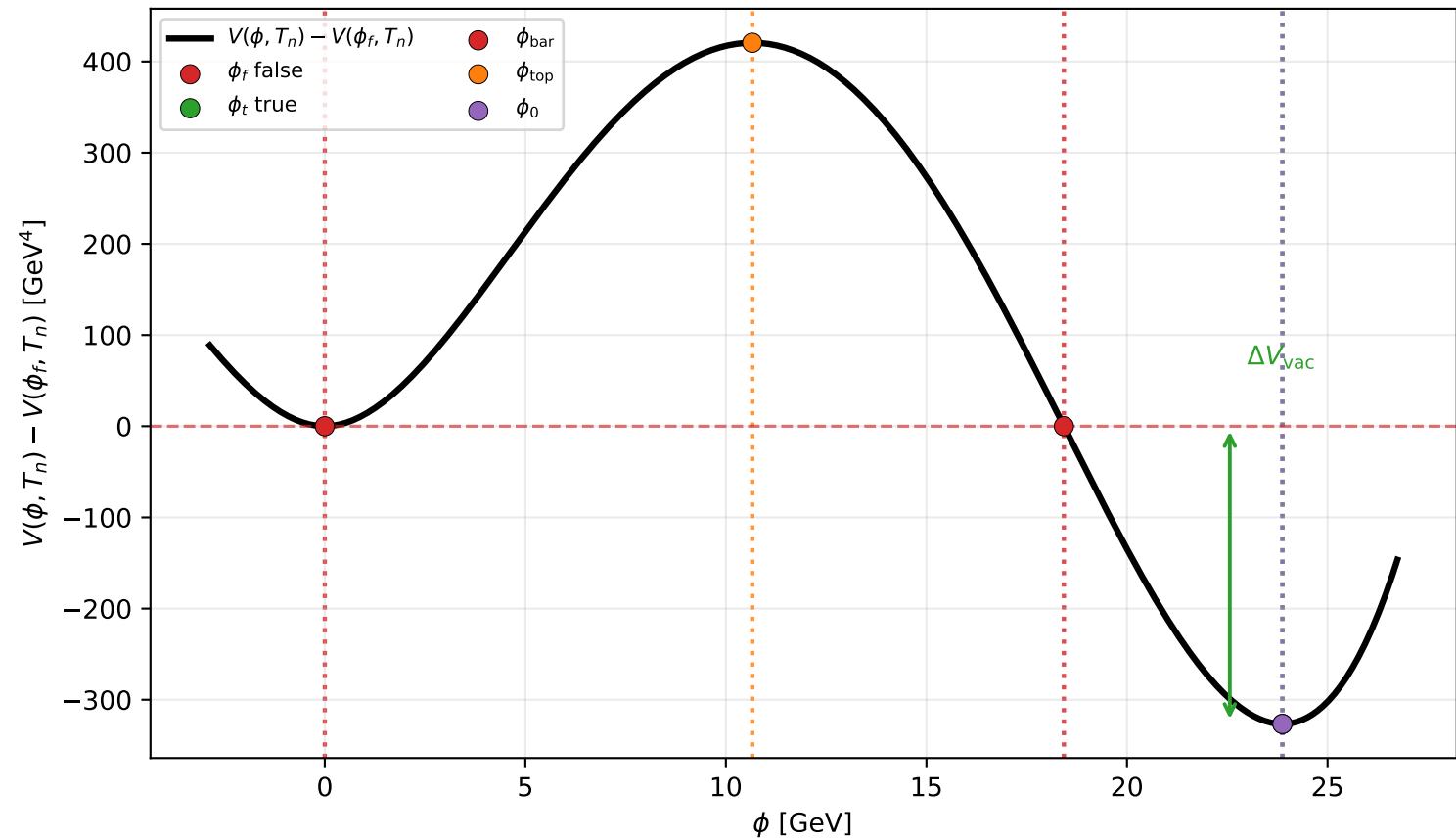
Example C1: potential geometry at T_n = 166.9 GeV
