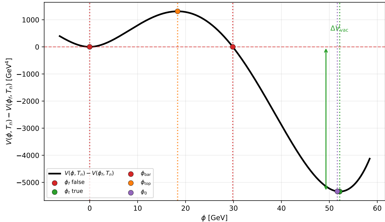
Example C1: potential geometry at T_n = 90.45 GeV
