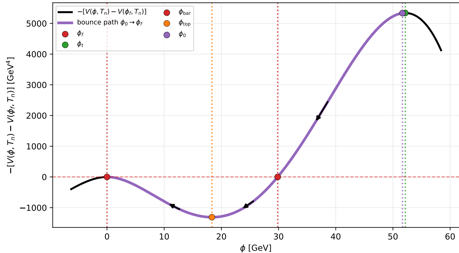
Example C2: inverted potential and bounce trajectory at T_n = 90.45 GeV
