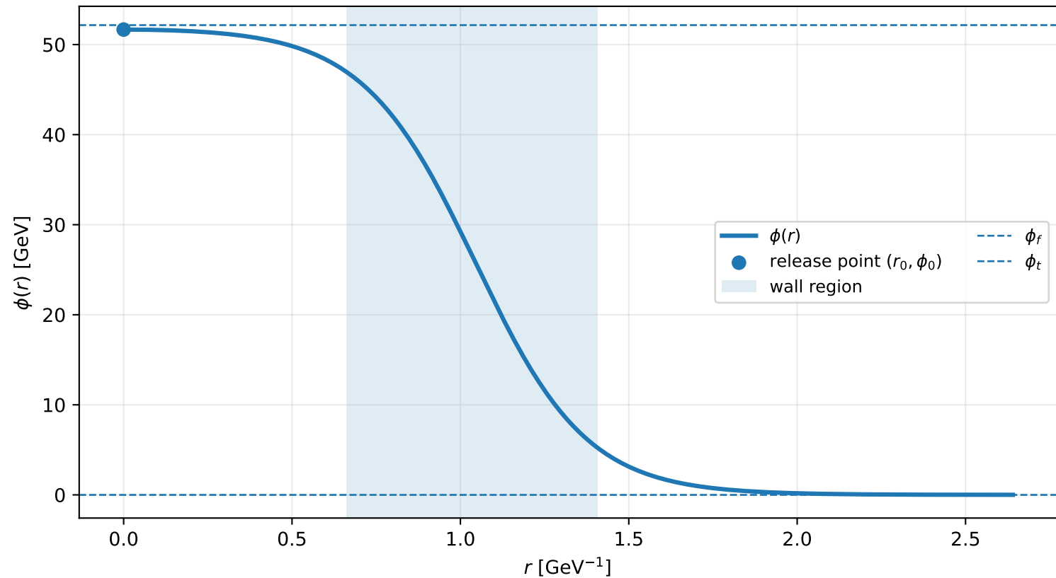
Example C3: bounce profile at T_n = 90.45 GeV
