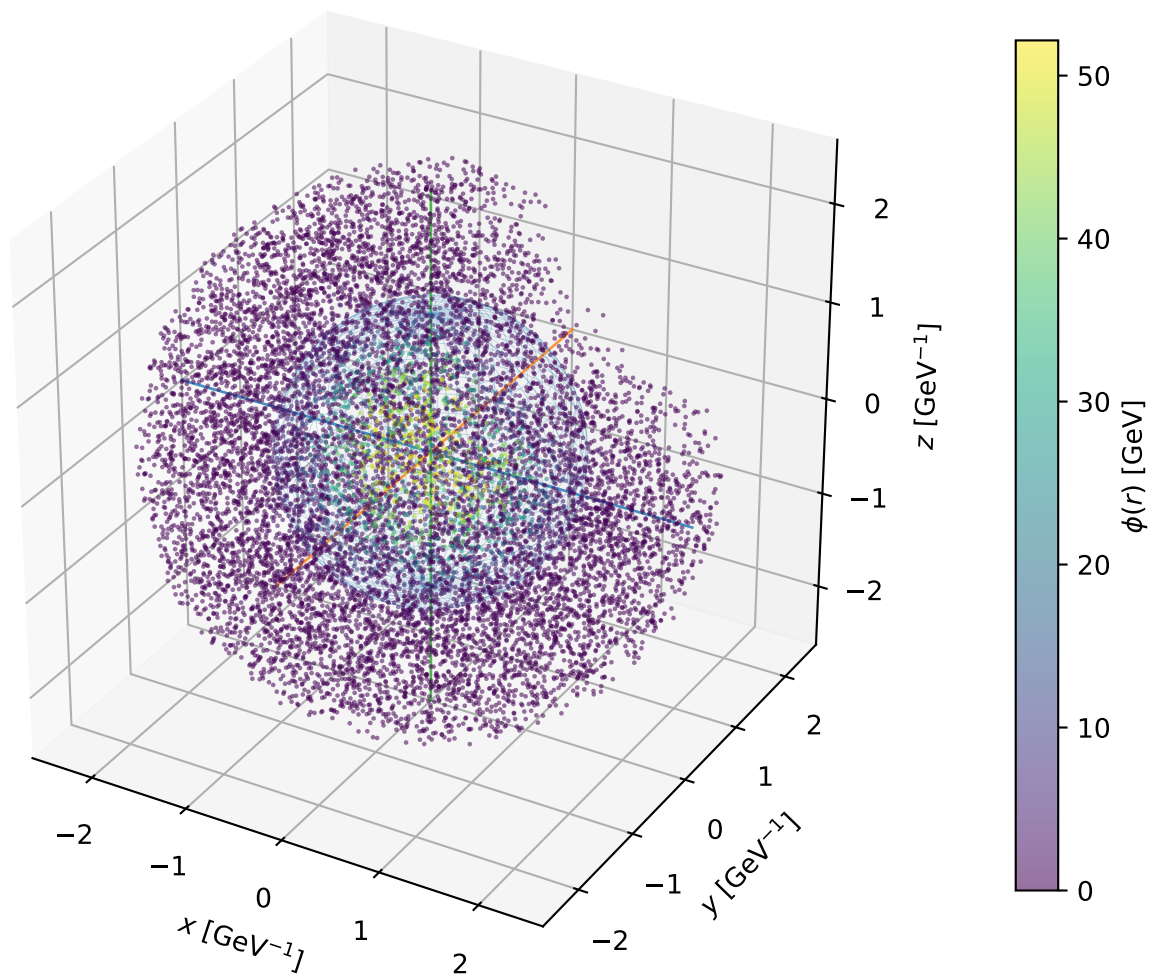
Example C5: 3D bubble profile at T_n = 90.45 GeV
