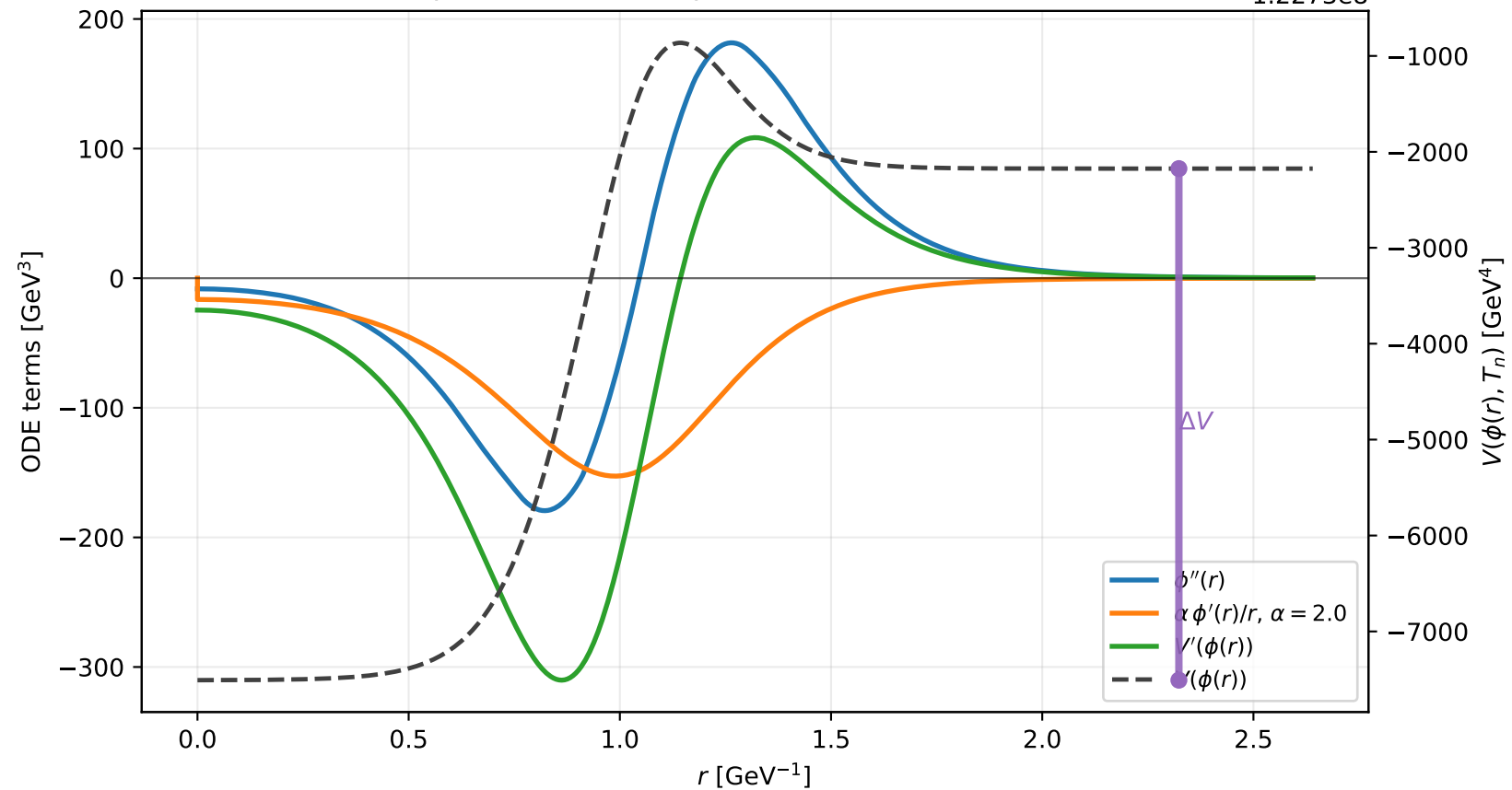
Example C7: bounce equation terms at T_n = 90.45 GeV
