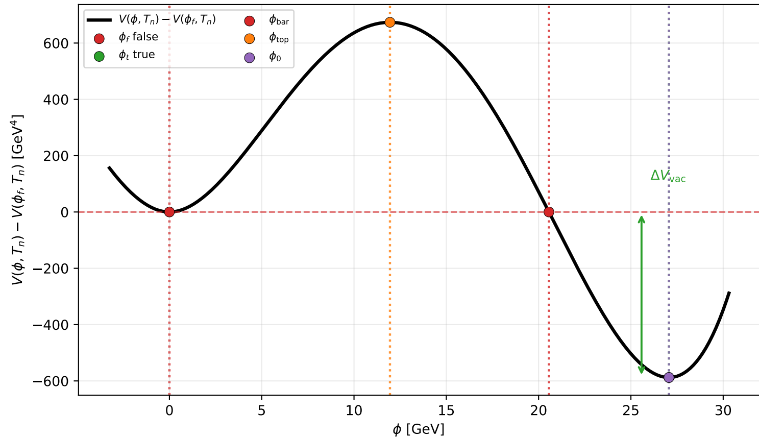
Example C1: potential geometry at T_n = 167 GeV
