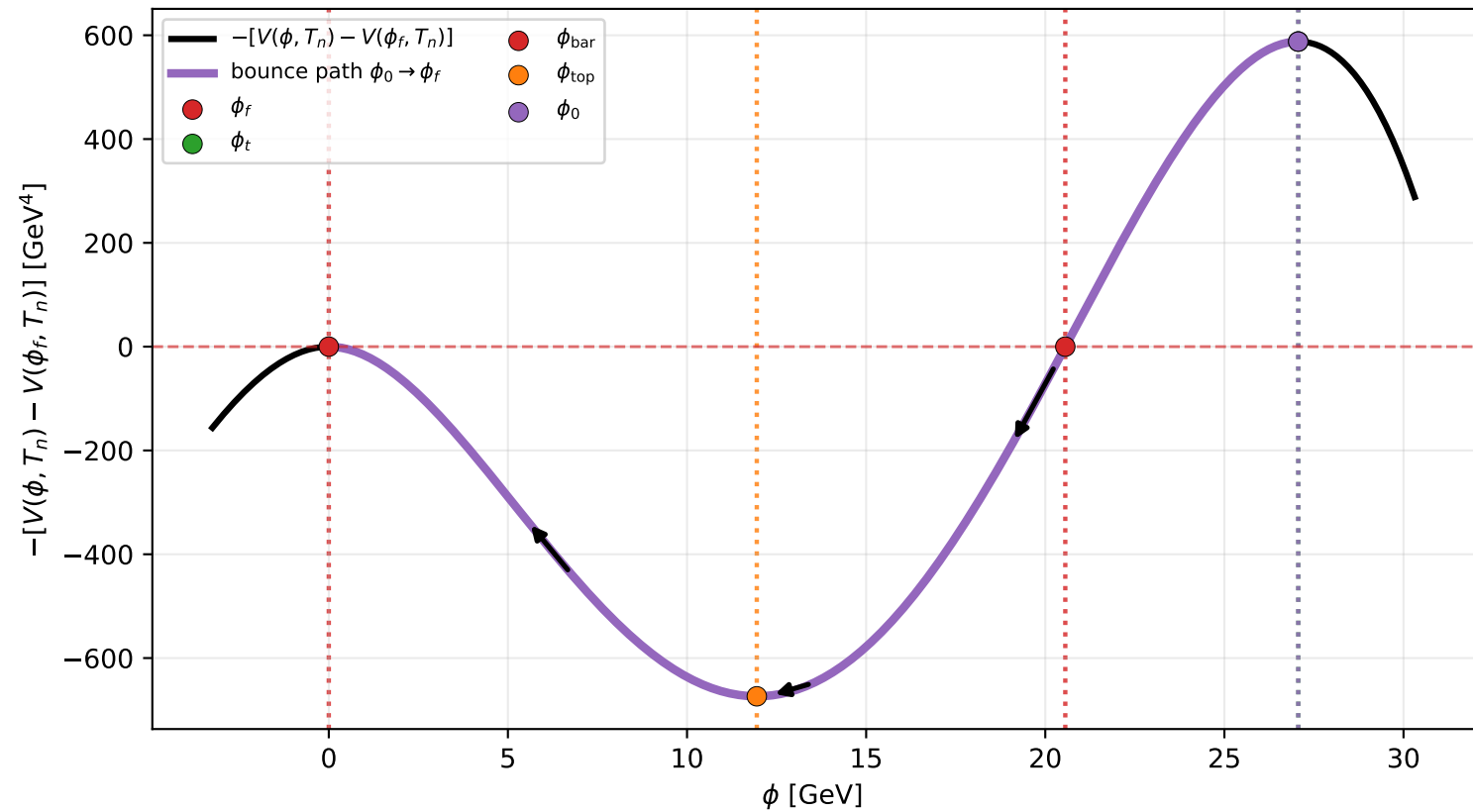
Example C2: inverted potential and bounce trajectory at T_n = 167 GeV
