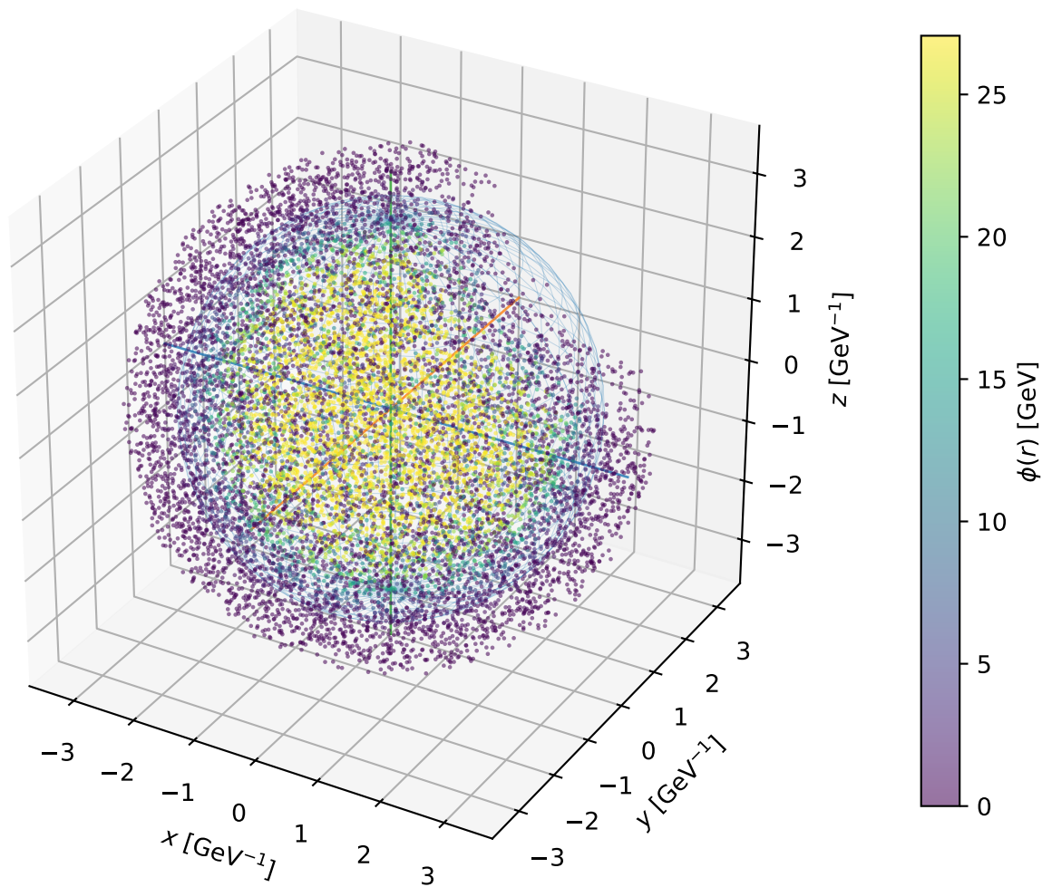
Example C5: 3D bubble profile at T_n = 167 GeV
