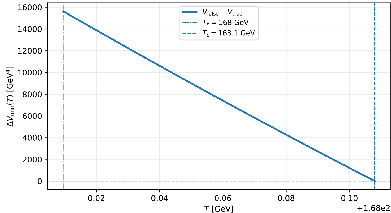
Example B5: free-energy difference between the two vacua
