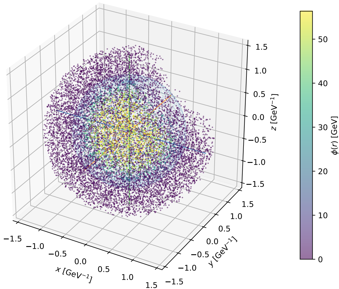
Example C5: 3D bubble profile at T_n = 168 GeV
