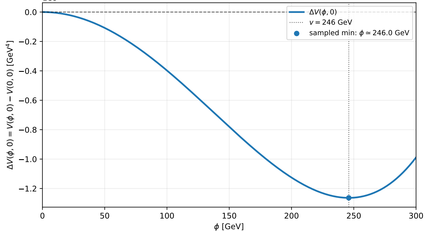
Example A1: zero-temperature potential near the electroweak vacuum without Gláuber measure, C=3.65 , \Lambda=1000 GeV, D=0.03 , m_h=125 GeV
