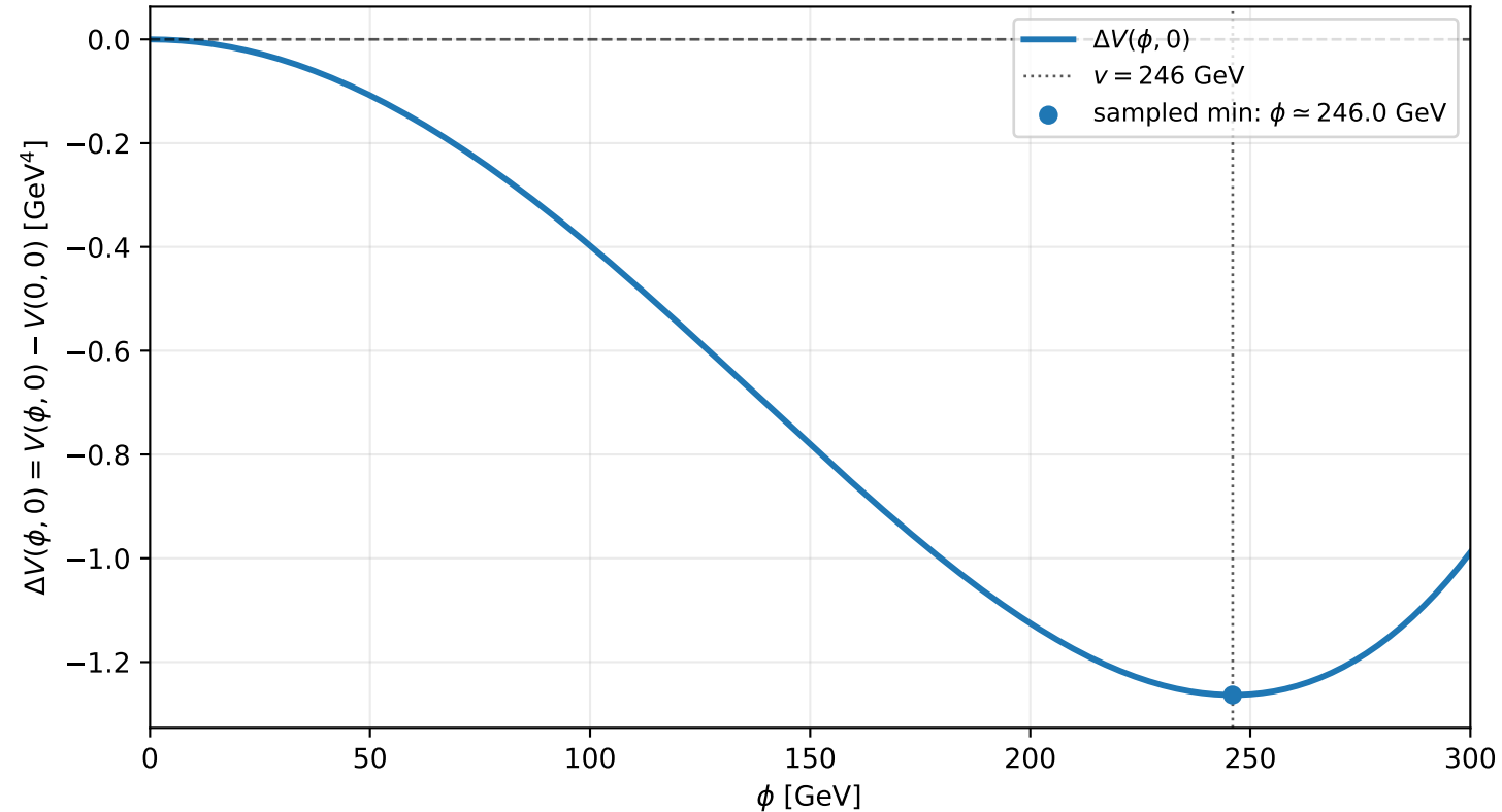
Example A1: zero-temperature potential near the electroweak vacuum without Gláuber measure, C=3.65 , \Lambda=1000 GeV, D=0.05 , m_h=125 GeV
