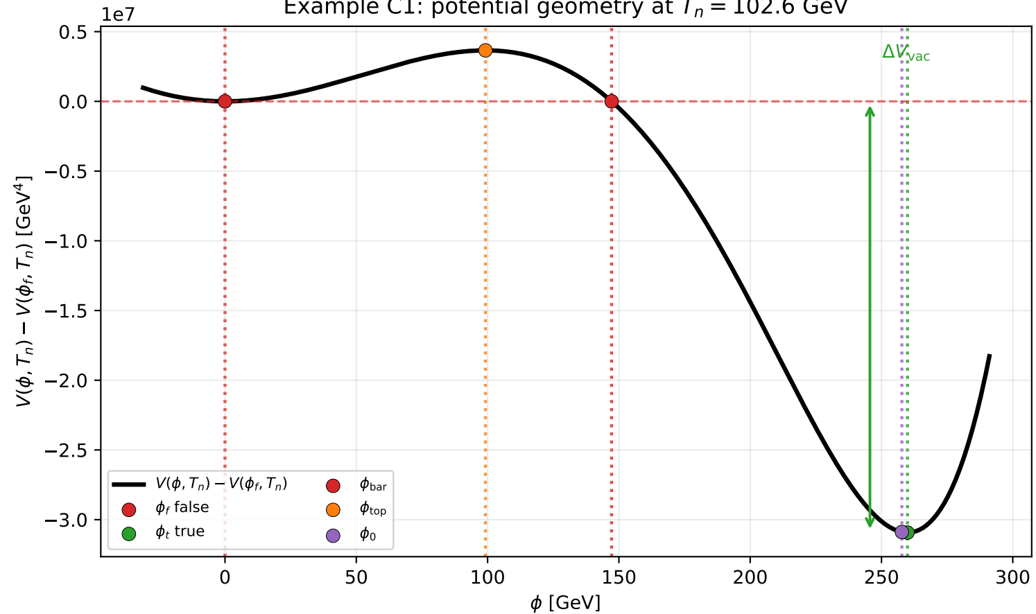
Example C1: potential geometry at T_n = 102.6 GeV
