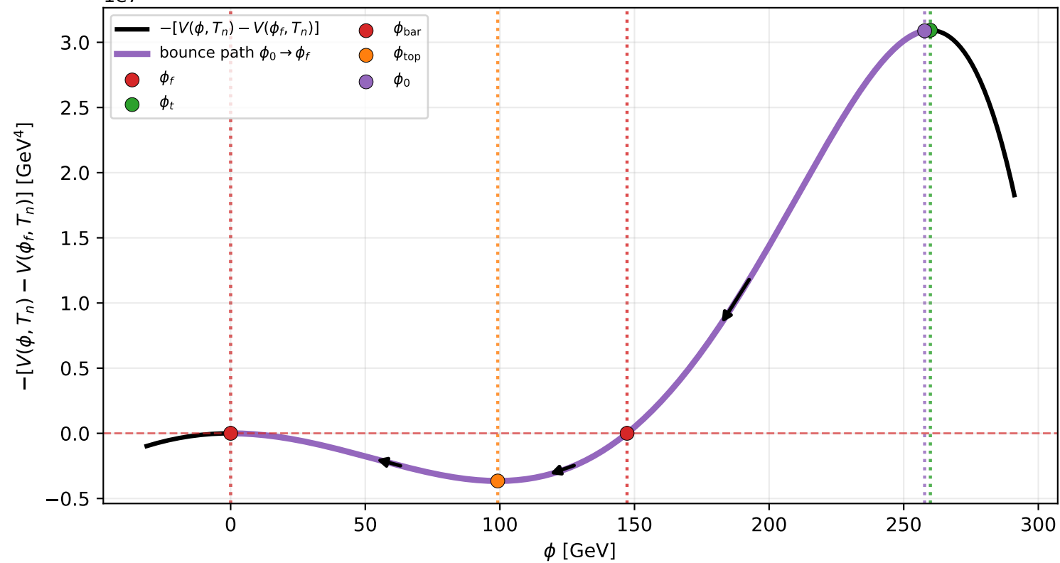
1e7 Example C2: inverted potential and bounce trajectory at T_n = 102.6 GeV
