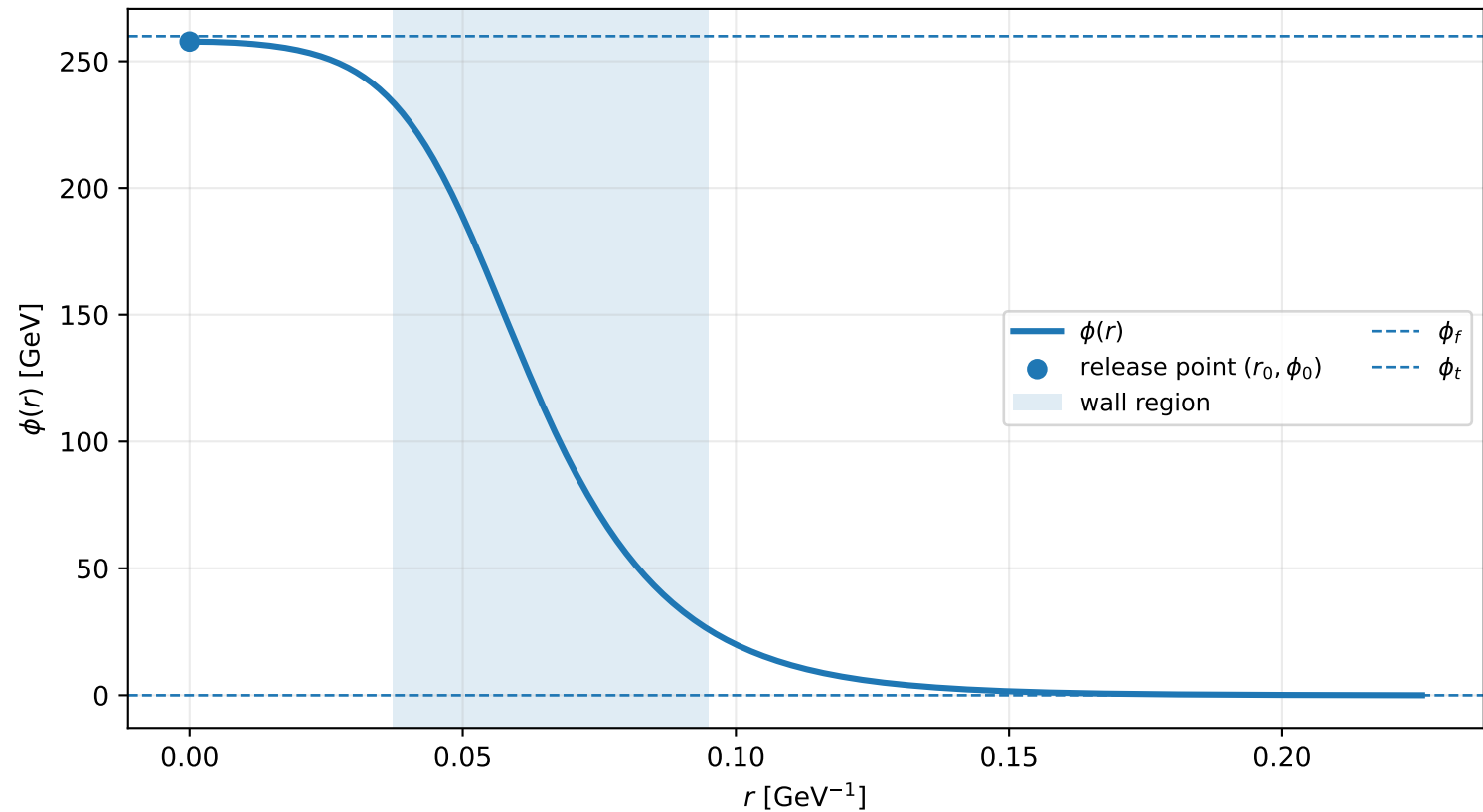
Example C3: bounce profile at T_n = 102.6 GeV
