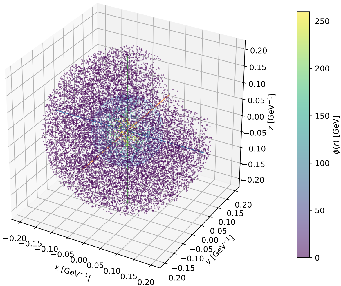
Example C5: 3D bubble profile at T_n = 102.6 GeV
