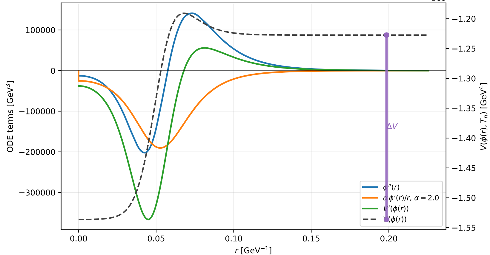
Example C7: bounce equation terms at T_n = 102.6 GeV
