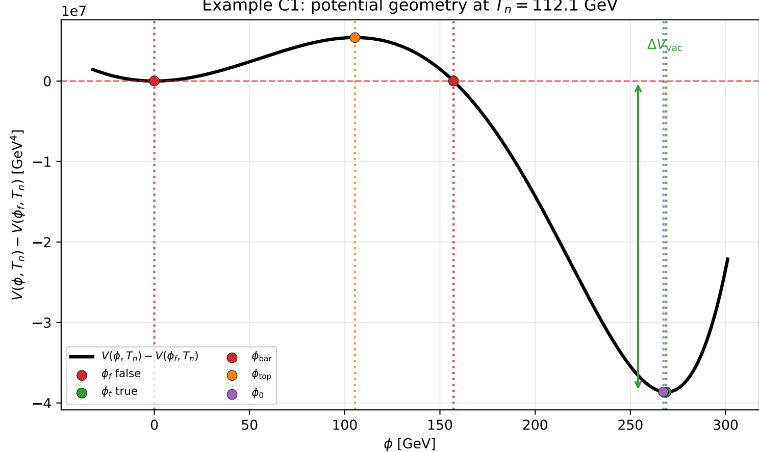
Example C1: potential geometry at T_n = 112.1 GeV
