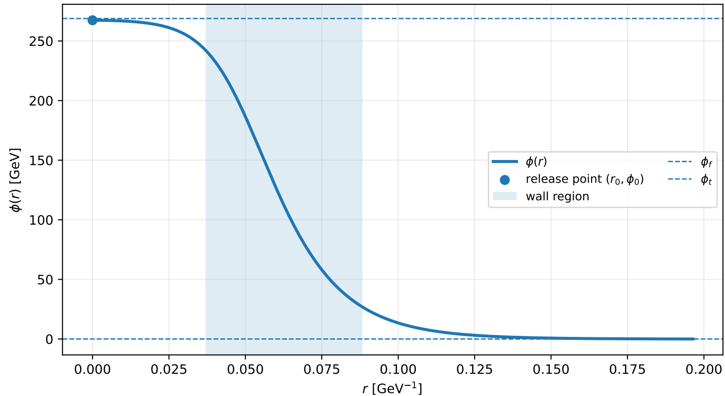
Example C3: bounce profile at T_n = 112.1 GeV
