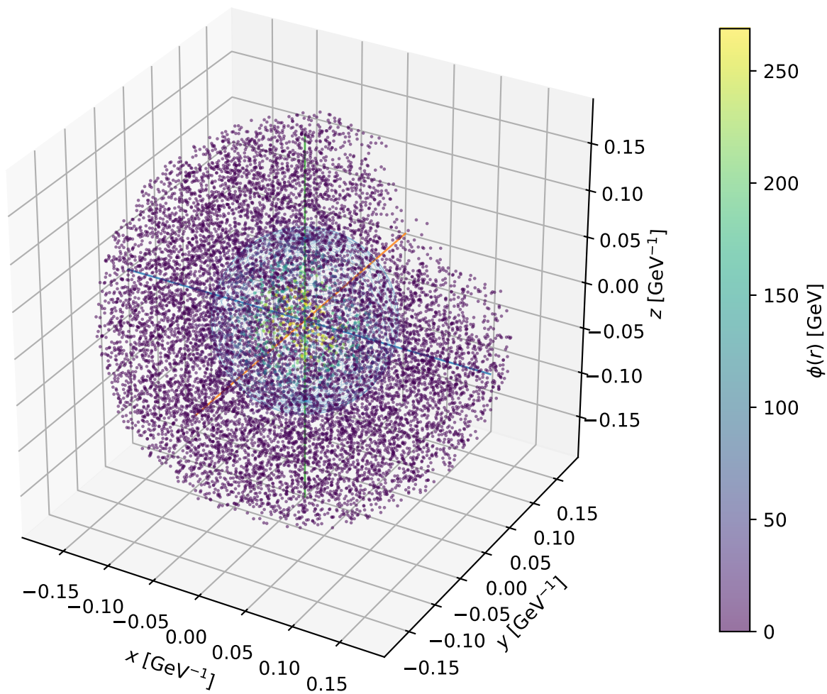
Example C5: 3D bubble profile at T_n = 112.1 GeV
