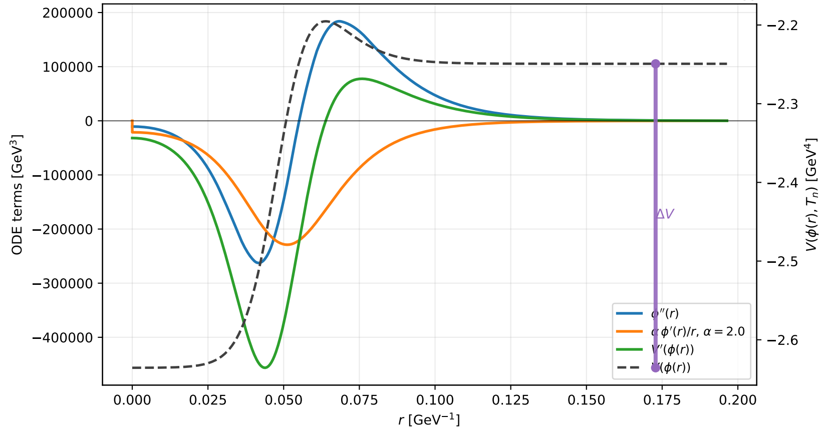
Example C7: bounce equation terms at T_n = 112.1 GeV
