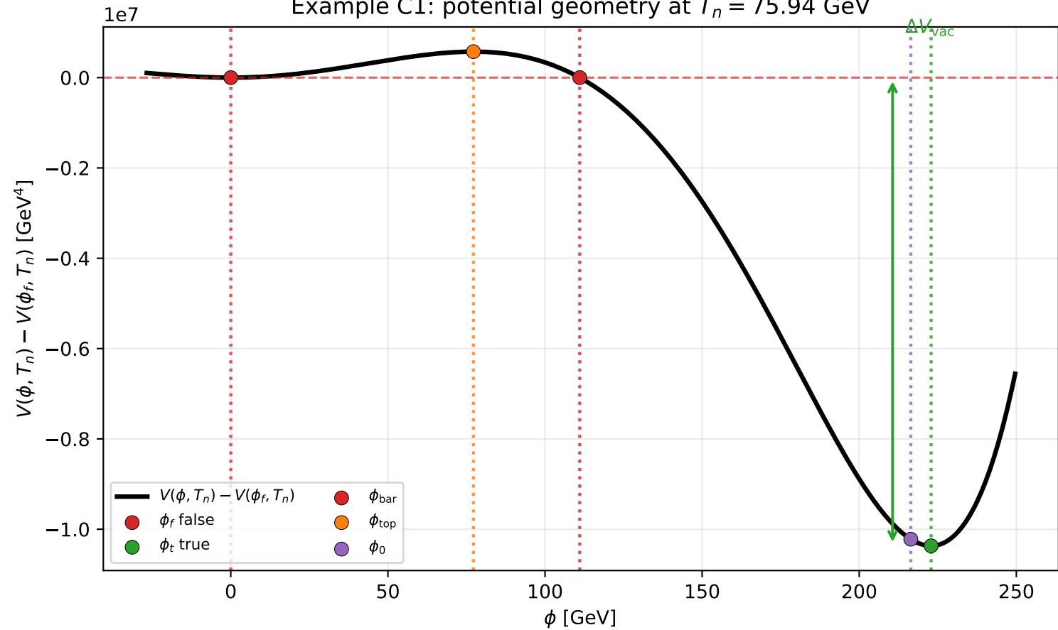
Example C1: potential geometry at T_n = 75.94 GeV
