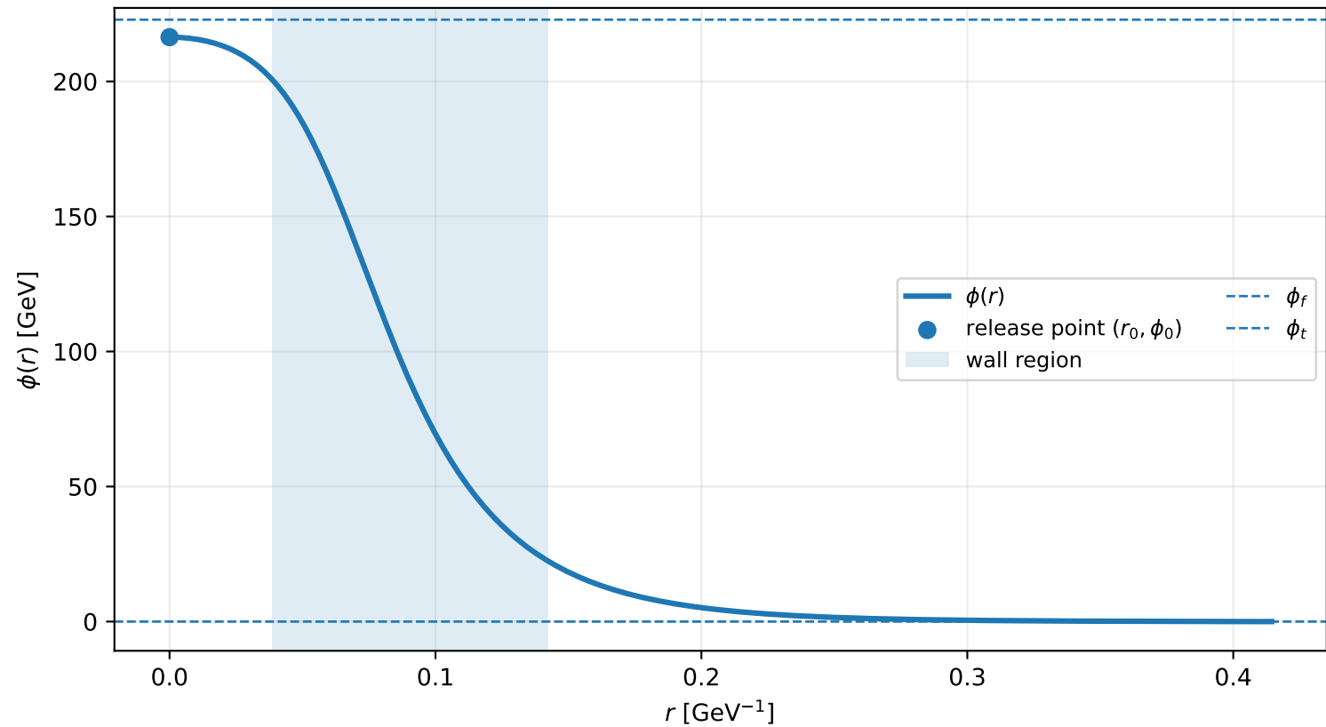
Example C3: bounce profile at T_n = 75.94 GeV
