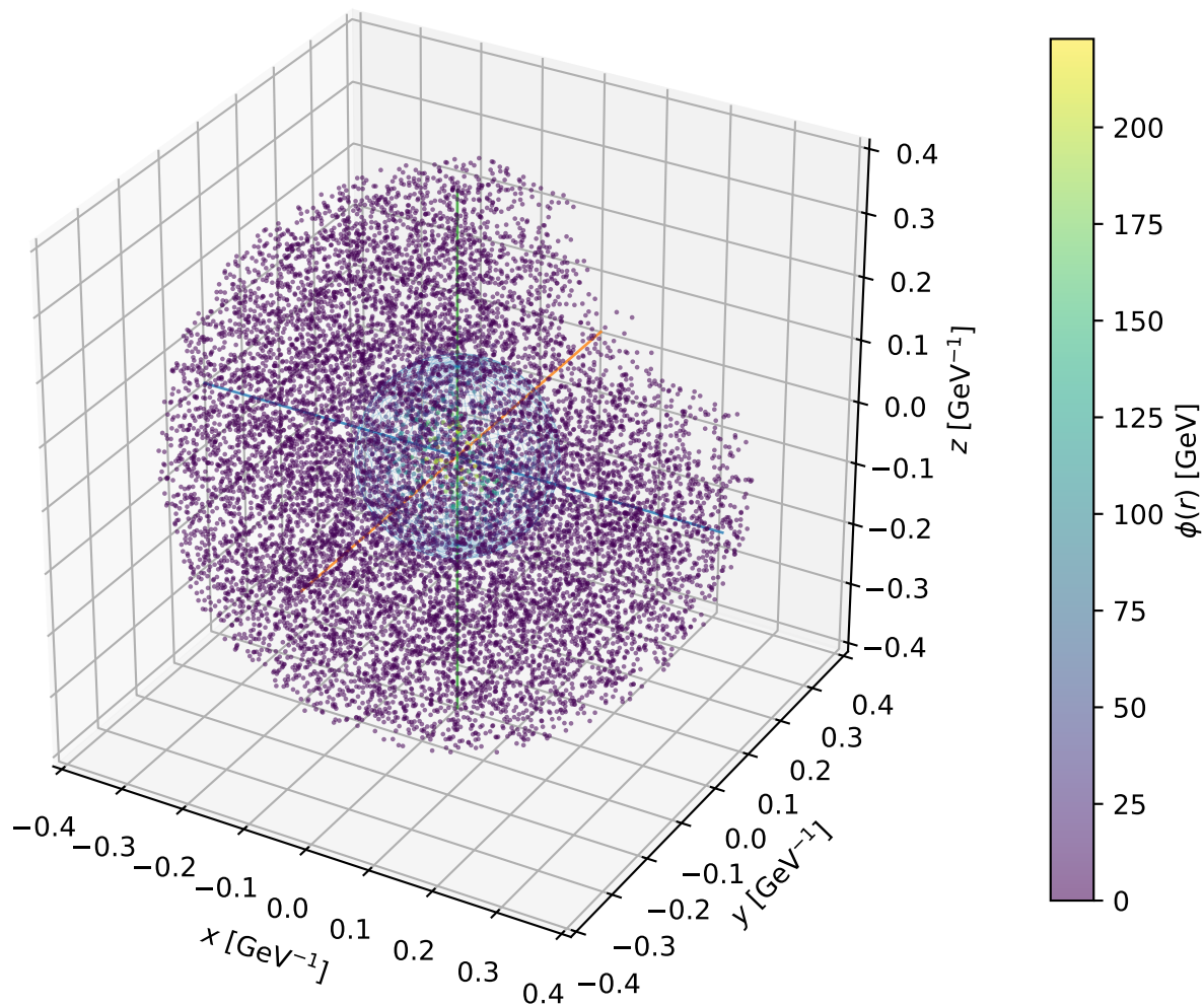
Example C5: 3D bubble profile at T_n = 75.94 GeV
