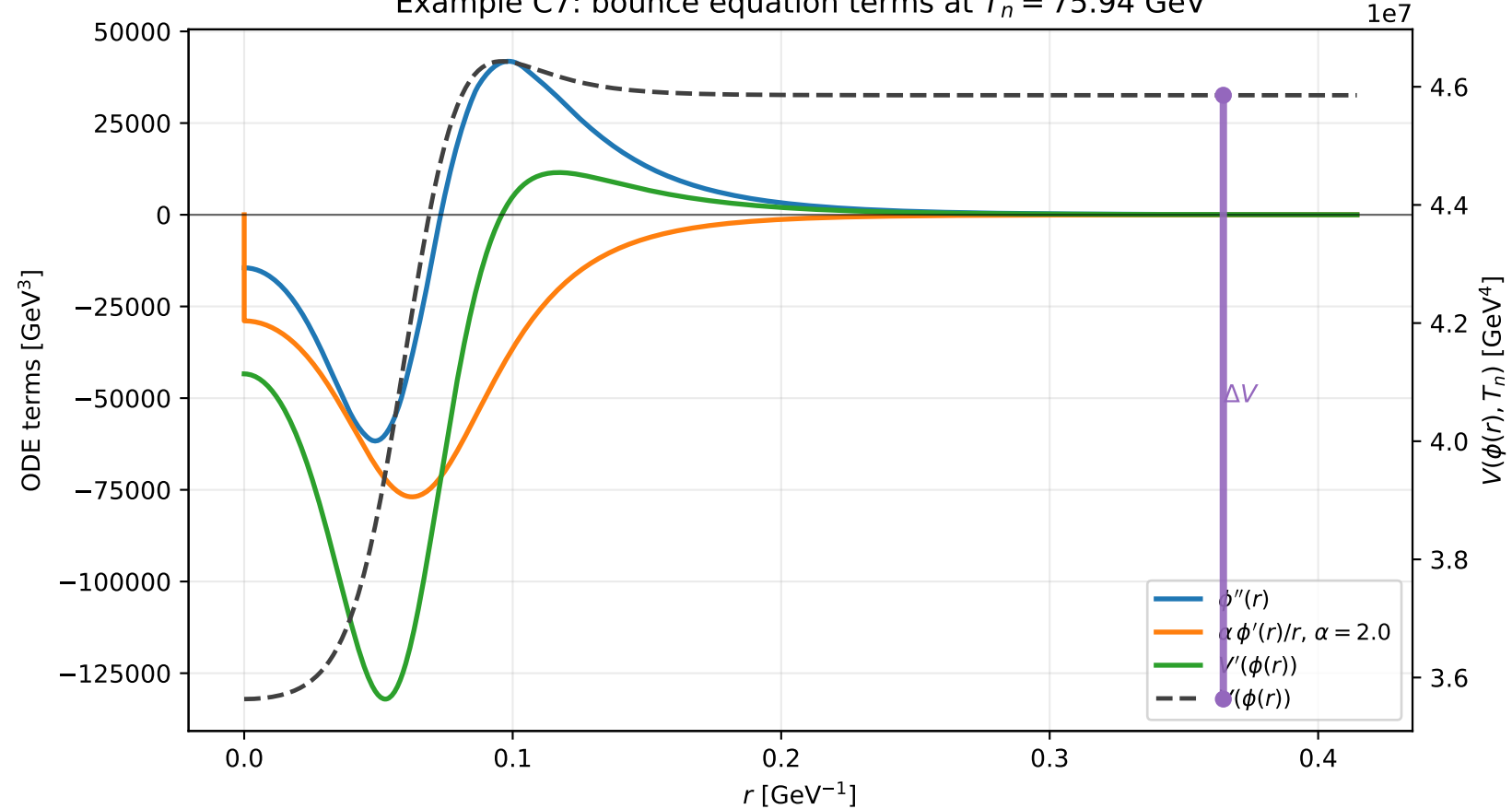
Example C7: bounce equation terms at T_n = 75.94 GeV
