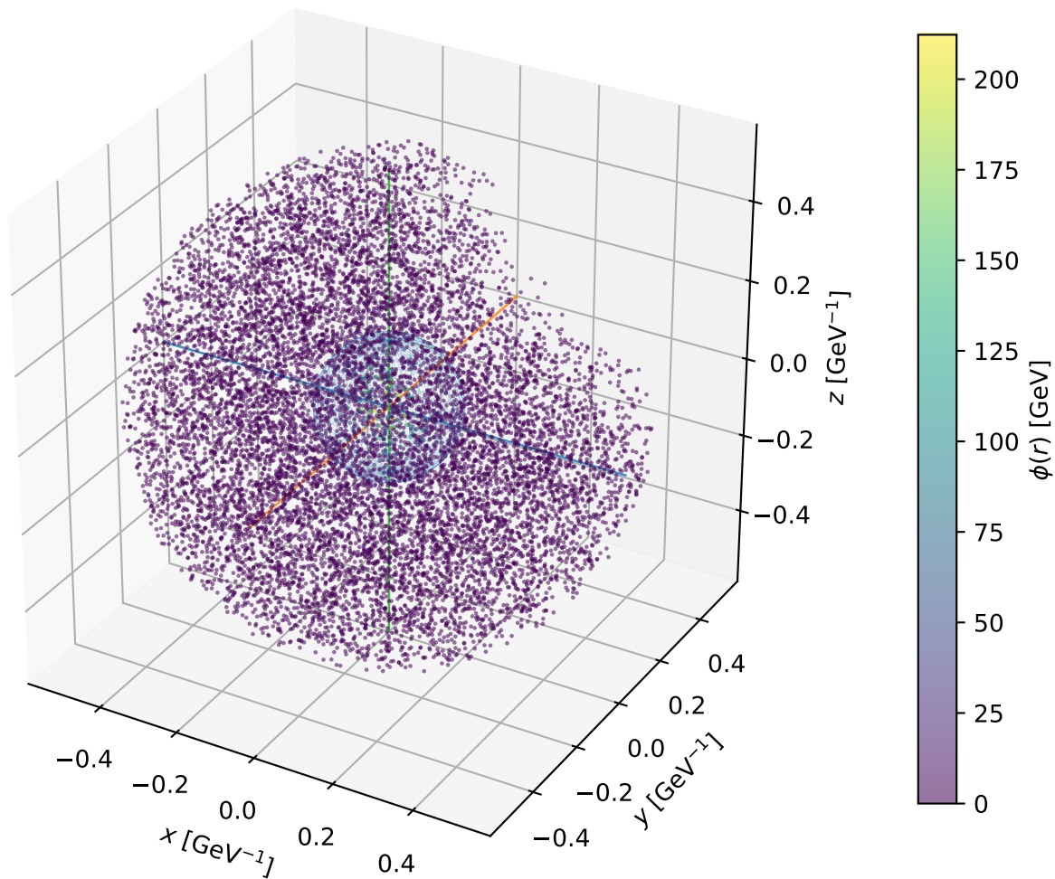
Example C5: 3D bubble profile at T_n = 71.58 GeV
