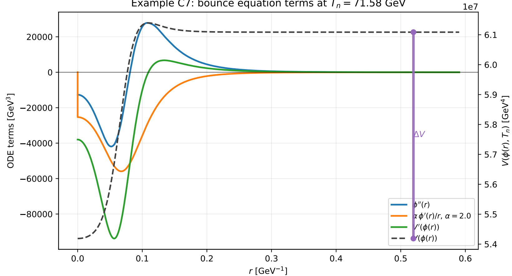
Example C7: bounce equation terms at T_n = 71.58 GeV
