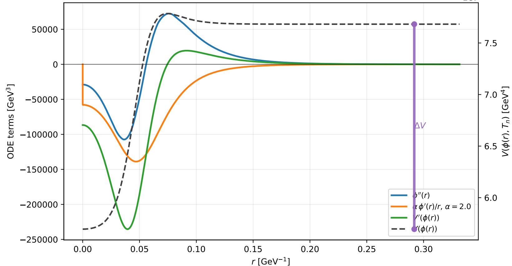
Example C7: bounce equation terms at T_n = 66.04 GeV
